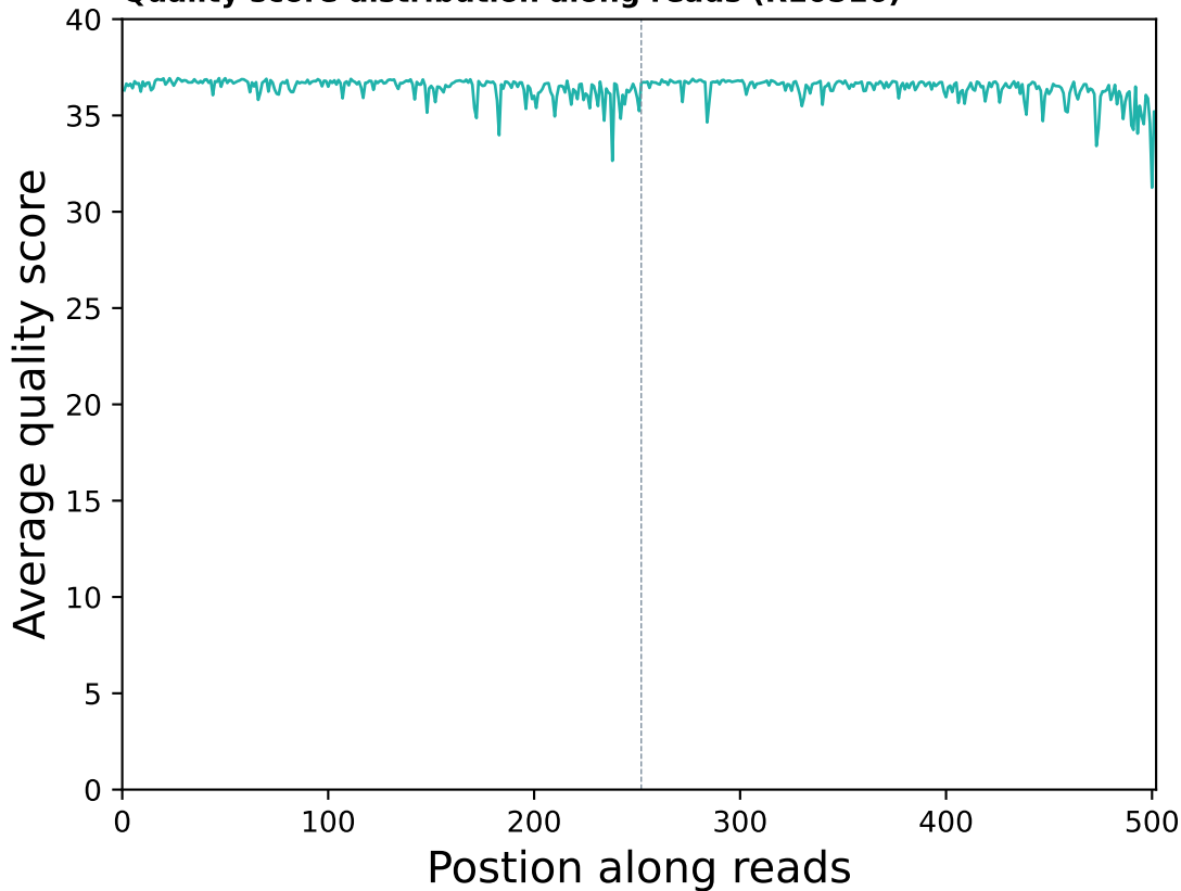
Quality score distribution along reads (R10516)
